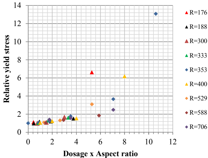
Fig. 7 Relative yield stress plotted as a function of the scaling for rigid fibers.
