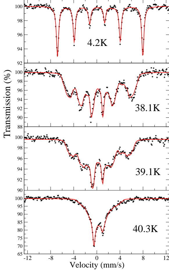
Figure 3: ^{57}\text{Fe} Mössbauer spectra in o\text{-YbMnO}_3\text{:Fe} at selected temperatures. The fits, shown by a solid red line, are as explained in the text.
