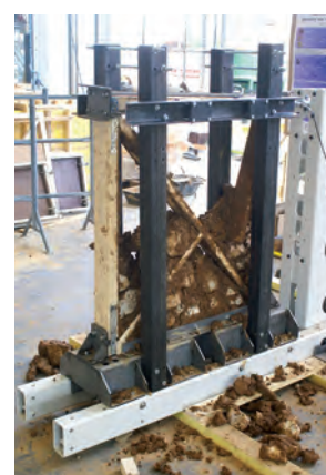
Above: a series of tests with the mini reaction wall on wall cell unit with different infill
