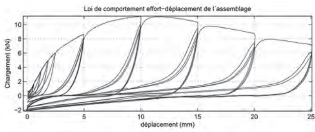
Different tests made to understand the behaviour of the structure under stress
