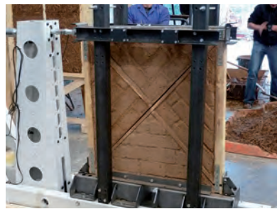
Above: a series of tests with the mini reaction wall on wall cell unit with different infill
