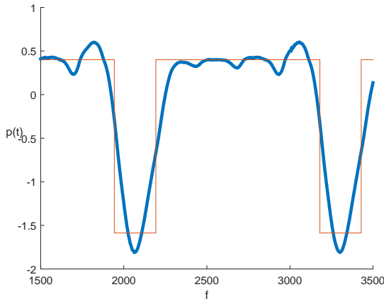
Figure 2: Example of waveshape for a soprano saxophone ( x_1 = 0.126\text{m} and \ell = 0.55\text{m} ) for the excitation parameters \gamma = 0.4 , \zeta = 0.65 (see Sect. 3.1). Thick line: RTC model; thin line: ideal Helmholtz motion model.
