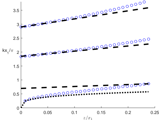
Figure 6: Frequency of the impedance maxima for the harmonics of the playing frequency with respect to the length z . \eta = 1 . Circles: numerical results of Eq. (33); dashed lines: Eqs. (37), for n = 1, 2, 3 ; dotted line: Eq. (38).
