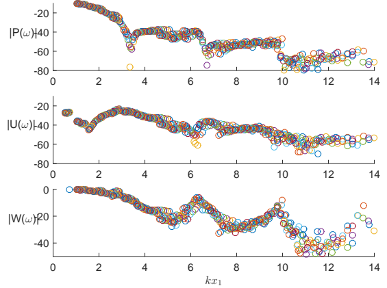
Figure 11: Input pressure P , input flow rate U , normalized output flow rate W for 32 values of the length \ell (logarithmic scale). x_1 = 0.126m , \ell = 0.33m to 0.64m \gamma = 0.4 , \zeta = 0.65 .
