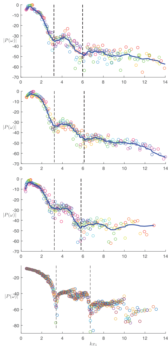
Figure 12: Mouthpiece pressure. From top to bottom: experimental results for a decreasing chromatic scale played on a soprano saxophone ( x_1 = .126\text{m} ), an alto saxophone ( x_1 = 0.196\text{m} ) and on a baritone saxophone ( x_1 = 0.301\text{m} ) The abscissa is kx_1 for the different saxophones, with different x_1 . Bottom: numerical results given by Fig. 11.
