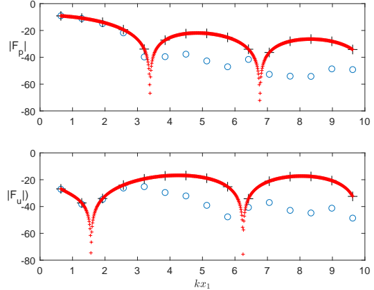
Figure 8: (top) Comparison between the input pressure P (ooo) for the harmonics of the playing frequency and the transfer function F_p (+++). x_1 = 0.126m , \ell = 0.4m , \gamma = 0.4 , \zeta = 0.65 . (bottom) Comparison between the input flow rate U (ooo) for the harmonics of the playing frequency and the transfer function F_u (+++). The small crosses (red online) represent the transfer functions for a continuous variation of the frequency.
