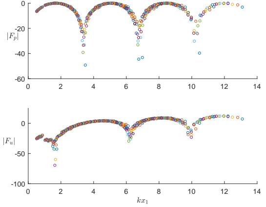
Figure 10: Transfer functions |F_p| and |F_U| for 32 values of the length \ell (logarithmic scale). x_1 = 0.126m , \ell = 0.33m to 0.64m \gamma = 0.4 , \zeta = 0.65 .
