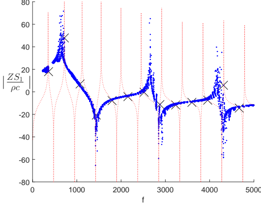
Figure 5: Values of the input impedance for the harmonics of 25 fundamental frequencies included in the first register of a soprano saxophone, corresponding to 25 values of the truncated cone length \ell . The impedance is calculated from Eq. (8), and plotted in dB. The frequency is in Hz. The calculation of the playing fundamental frequencies uses the results presented in Fig. 4 for \gamma = 0.4 ; \zeta = 0.65 . In order to exhibit an example, the results for one length is indicated by a cross 'X' for \ell=0.352 m, and the complete impedance curve for this length is drawn by a thin line. .
