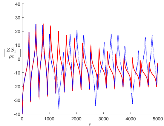
Figure 3: Example of input impedance modulus curves (in dB) for x_1 = 0.126m and \ell = 0.55m . Solid line: RTC model; dotted line: approximation corresponding to the cylindrical saxophone model (ideal Helmholtz motion).
