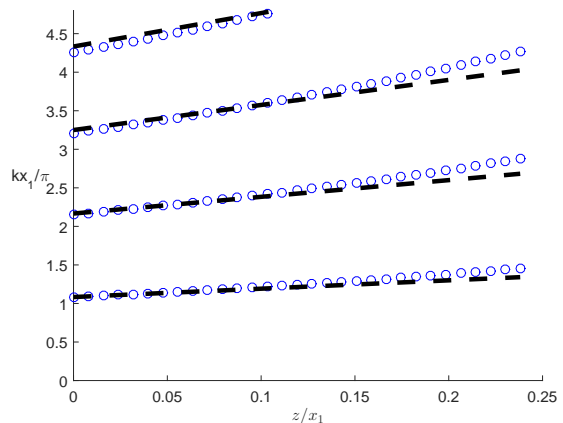
Figure 7: Frequency of the impedance minima for the harmonics of the playing frequency with respect to the length correction z . Circles: numerical results; dashed lines: Eq. (39) for \sigma = 1/12 .
