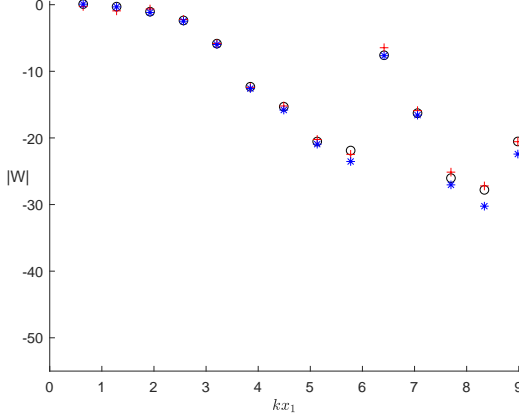
Figure 9: Normalized output flow rate |W| . Eq. (19) is computed in 3 ways: direct computation of the spectrum from the time-domain (**), |P/F_p| (ooo), |U/F_U| (+++). Logarithmic scale (for a cylindrical saxophone, \log_{10}(|W|) vanishes). x_1 = 0.126m , \ell = 0.4m , \gamma = 0.4 , \zeta = 0.65 .
