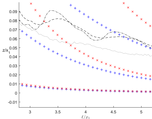
Figure 4: Length z ( -z is the length correction) related to the playing frequency represented by the ratio \ell/x_1 for several values of the length \ell of the truncated cone (simulation results). When \ell varies from 0.35 m to 0.67 m, the ratio \beta decreases from 0.26 to 0.16. x_1 = 0.126 m. Thin lines: dotted ( \gamma = \zeta = 0.4 ), mixed ( \gamma = 0.45 ; \zeta = 0.85 ), dashed ( \gamma = 0.4 ; \zeta = 0.65 ). +++ Formula (25), for one, two, three terms of the series (from bottom to top). xxx Formula (26), for one, two, three terms of the series (from bottom to top).
