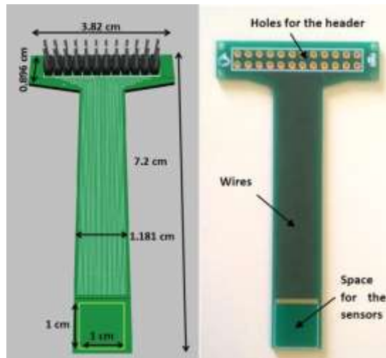
Fig. 2 The PCB designed for the sensor chip connection.
