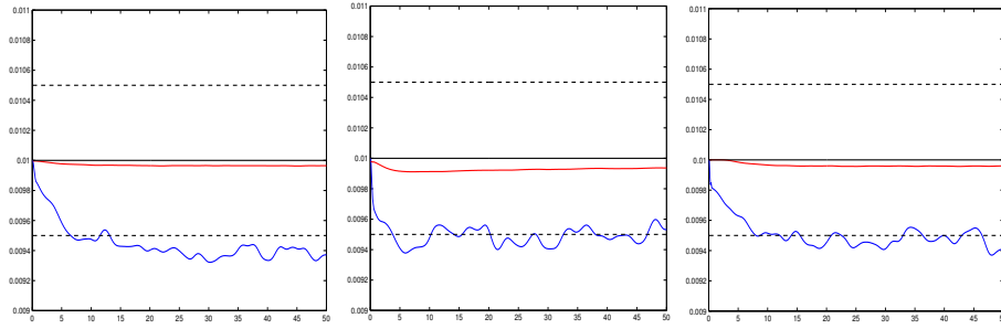
FIGURE 4. Same as Figure 3 except that \alpha = 0.01 .
