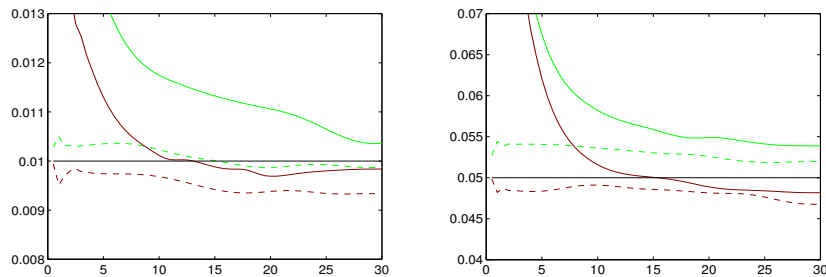
FIGURE 6. The process considered here has covariance \rho(t) = \exp(-t^{1.95}) ; Exact level of a test constructed for a nominal level of \alpha = 1\% (left) or \alpha = 5\% (right) using the Pickands method . Our numerical computation uses the lower bound of MGP, thus it provides an under estimation. The meaning of the colours and dashed lin is the same as in Figure 5.
