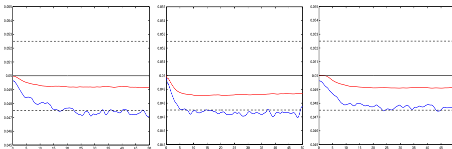
FIGURE 3. Exact level of a test constructed for a nominal level of \alpha = 5\% using the Rice method (see Section 2). An upper bound (red line) and a lower bound (blue line) of the level are computed by the program MGP (see Section 3.1.1). From left to right, the processes considered have covariance function \rho(t) = \exp(-t^2/2) , \rho(t) = 1/\cosh(t) and \rho(t) = \text{sinc}(\sqrt{3}t) .
