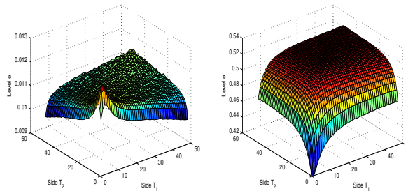
FIGURE 12. Same as Figure 11 except that : The covariance is always \rho(t) = \exp(-t^2/2) and \alpha = 0.01 (left) and \alpha = 0.5 (right)
