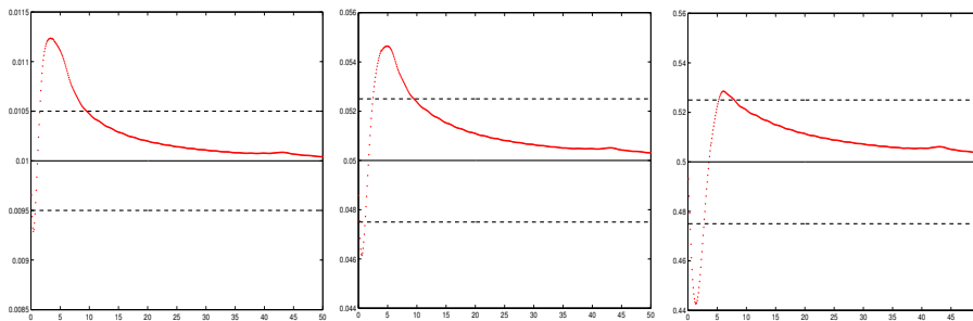
FIGURE 13. Exact level of a test constructed for a nominal level of, from left to right, \alpha = 1\% , \alpha = 5\% and \alpha = 50\% , using the Euler characteristic method (see Section 2) on subsets of the diagonal of [0, 50]^2 . The upper bound presented here is computed by the program MAXNSGP2 (see Section 3.1.1) and the process considered has covariance function \rho(t) = \exp(-t^2/2) .
