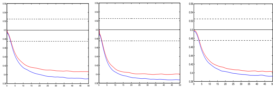
FIGURE 9. Exact level of a test constructed for a nominal level of \alpha = 50\% using the Rice method (see Section 2). An upper bound (red line) and a lower bound (blue line) of the level are computed by the program MGP (see Section 3.1.1). From left to right, the processes considered have covariance function \rho(t) = \exp(-t^2/2) , \rho(t) = 1/\cosh(t) and \rho(t) = \text{sinc}(\sqrt{3}t) .
