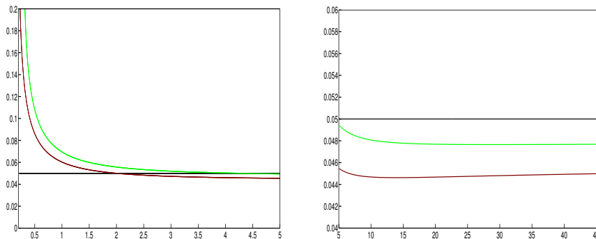
FIGURE 1. Exact level of a test constructed for a nominal level of \alpha = 5\% using the Pickands method and the Ornstein-Uhlenbeck process. On the left: small intervals, on the right: large intervals (see Section 2). The level corresponding to equation (2) is given in brown while the one of equation (3) is given in green. Both are computed thanks to the pou program (see Section 3.1.1)
