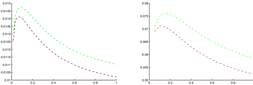
FIGURE 8. Zoom of Figure 5 for the dotted lines and small values of T .
