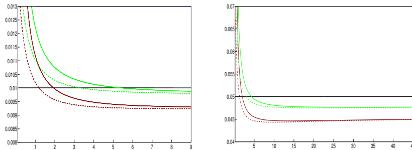
FIGURE 5. Exact level of a test constructed for the Ornstein-Uhlenbeck process and a nominal level of \alpha = 1\% (left) or \alpha = 5\% (right) using the Pickands method and the program pou . The level corresponding to equation (2) is given in brown, the one of equation (3) is given in green while the modified versions including \bar{\Phi}(u) are given in dashed.
