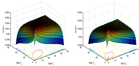
FIGURE 11. Exact level of a test constructed for a nominal level of \alpha = 5\% using the Euler characteristic method (see Section 2) on subsets of [0, 50]^2 . The upper bound presented here is computed by the program MAXNSGP2 (see Section 3.1.1) and the processes considered have covariance function \rho(t) = \exp(-t^2/2) (left) and \rho(t) = (1 + \|t\|)\exp(-\|t\|) (right).
