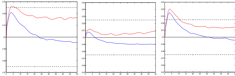
FIGURE 10. Exact probability of M_T to be above the approximate median computed with the Poisson method (see Section 2). An upper bound (red line) and a lower bound (blue line) of the probability are computed by MGP (see Section 3.1.1). From left to right, the processes considered have covariance function \rho(t) = \exp(-t^2/2) , \rho(t) = 1/\cosh(t) and \rho(t) = \text{sinc}(\sqrt{3}t) .
