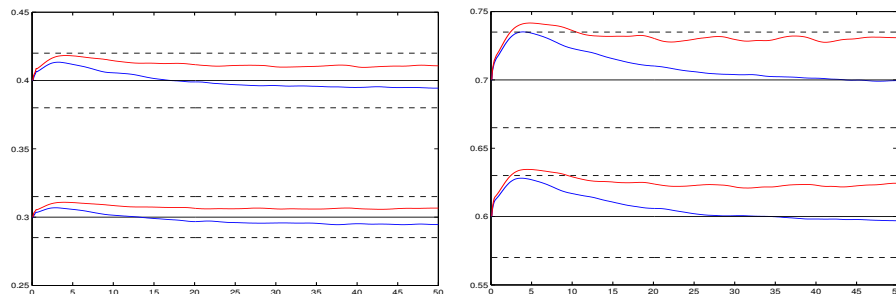
FIGURE 14. Exact probability of M_T to be above the approximate 1 - 0.40 (left top); 1 - 0.70 (right top) 1 - 0.30 (left bottom) 1 - 0.60 (right bottom) fractile computed with the Poisson method (see Section 2) on subsets of [0, 50] . An upper bound (red line) and a lower bound (blue line) of the level are computed by the program MGP (see Section 3.1.1). The process considered has covariance function \rho(t) = \exp(-t^2/2) .
