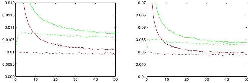
FIGURE 7. Same as Figure 6 except that (a) the covariance is now \rho(t) = \exp(-t^2/2) , (b) the computation uses the upper-bound of MGP which is known to be precise
