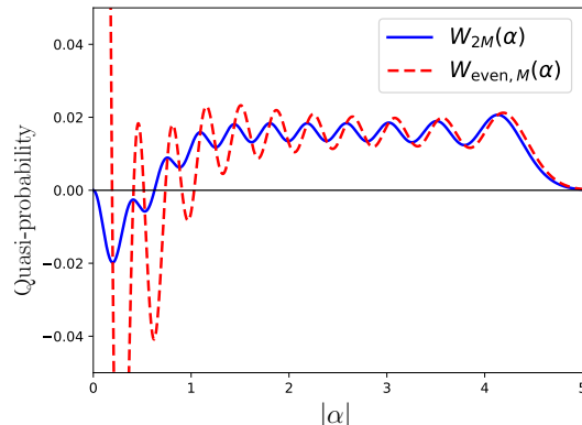
FIGURE 1. Colour online. Plots of the Wigner functions of \rho_{2M} (solid line) and of \rho_{\text{even},M} (dashed line) as a function of |\alpha| for M = 10 . Both states have comparable photon number: \text{Tr}(\rho_{2M}a^\dagger a) = M + \frac{1}{2} , \text{Tr}(\rho_{\text{even},M}a^\dagger a) = M + 1 . The oscillations in the Wigner function of one are visibly much more pronounced than in the other, as detailed in the text.
