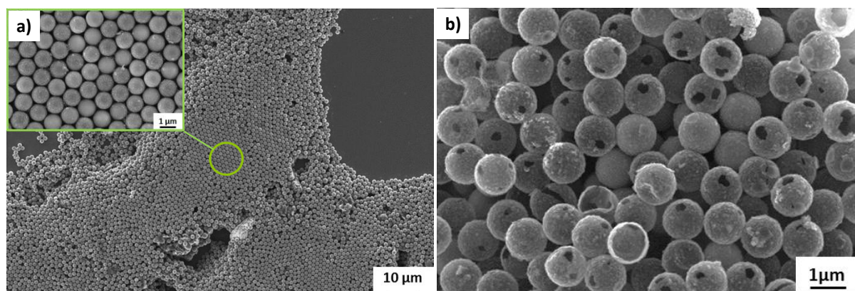
Figure 16 : a) FE-SEM images of self-assembly of graphite nanoflakes coated particles deposited on silicon substrate exhibiting a hexagonal structure. Other MPCVD parameters: total pressure 12.5 mbar, flow rate 10 sccm, microwave power 180 W, 30 % of methane during 15 minutes. b) FE-SEM image of graphite nanoflakes shells obtained after a dissolution of silica core by basic solution.
