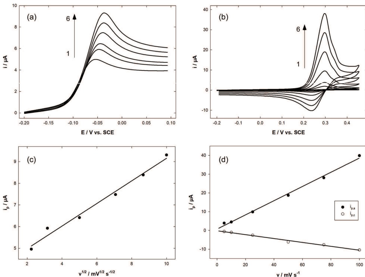
Fig. 2. Linear (Figure 2.a.) and cyclic (Figure 2.b.) voltammograms recorded with Au-PEDOT electrode in 0.1 \text{ molL}^{-1} PBS pH 7.0 containing 10^{-3} \text{ molL}^{-1} AA (Figure 2.a.) and 10^{-3} \text{ molL}^{-1} UA (Figure 2.b.). Variation of the potential scan rate: (1) 5; (2) 10; (3) 25; (4) 50; (5) 75 and (6) 100 \text{mV s}^{-1} . Influence of the potential scan rate on AA oxidation peak current (Figure 2.c) and on both oxidation/reduction UA peak currents (Figure 2.d).
