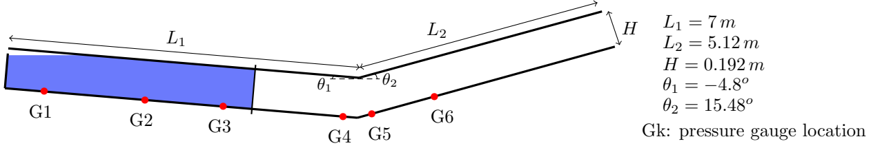
FIGURE 3.13. Configuration and initial condition and for the Aureli et al. test case.
