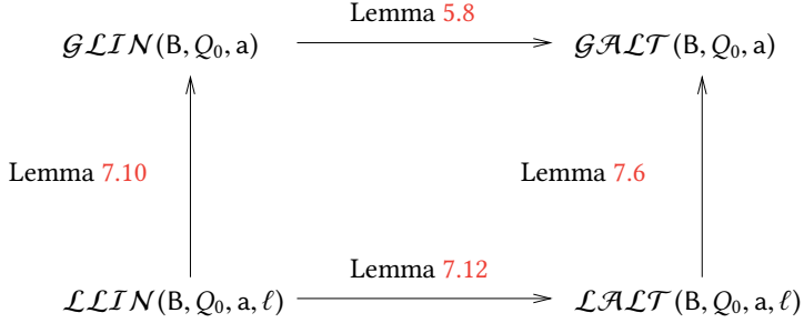
Fig. 9. Implication relations between deadlock-freedom conditions.
