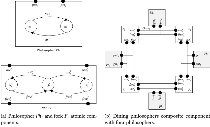
Fig. 1. Dining philosophers.
