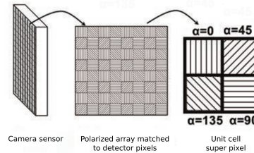
Fig. 1. Structure of DoFP sensors: in a single shot, four polarized images are acquired, each of them with a different polarized angles.
