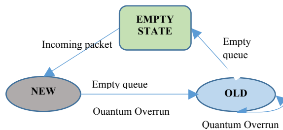
Figure 1. FQ-CoDel State Machine
