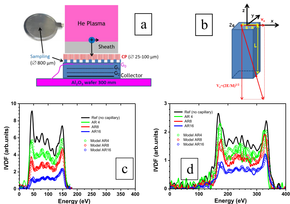
FIG. 1. (a) Schematic of the 4 grid RFEA sensor on the 300 mm diameter wafer. The capillary plate (CP) is lying on the \text{Al}_2\text{O}_3 cover of the sensor. (b) A square shape hole, which is used to model the cylindrical holes of radius R of real CP, has an aspect ratio of L/2a , where 2a is the square side dimension. The ion vertical velocity is related to their energy E . In this example, the ion transverse velocity v_x is the maximum possible allowing it to pass through the hole. (c) and (d) IVDF measured without capillary plate (black curve) and with CP4, CP8, and CP16 (plain lines). He plasma at 10 mTorr with (c) 750 W ICP power and 200 W rf bias power and (d) 400 W ICP power and 300 W rf bias power. Open symbols are obtained from Eq. (4) with the Reference IVDF as an input and assuming T_i = 0.27 eV.
