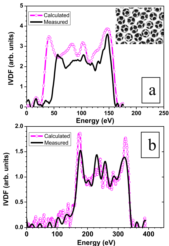
FIG. 3. (a) and (b) The IVDF measured for plasma conditions of Fig. 1(c) and 1(d), respectively, after passing through the stack CPs (black). The magenta symbols are obtained by using Eq. (4) to predict how the incoming IVDF (measured through CP4) should evolve after passing through a CP8. Inset: top view optical image of the CP4 + CP8 stack.
