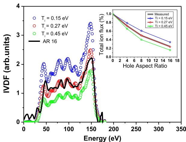
FIG. 2. IVDF measured through CP16 (black) and fit from Eq. (4) using three different T_i (0.15, 0.27, and 0.45 eV). The inset shows the variations of the total ion flux as a function of AR together with the result of Eq. (4) for the same three T_i .
