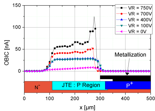
Figure 7. OBIC vs. beam position for several voltage reverse voltages (structure b) using the green laser.
