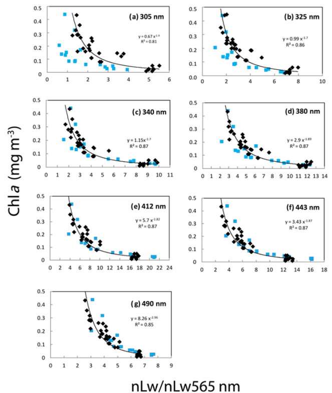
Figure 11. Correlations between the Chl a (fluorimetry) and the ratio of nL_w(\lambda)/nL_w(565\ nm) at different UV and visible wavelengths. Equations and determination coefficient ( r^2 ) of the power law are indicated for each wavelength: (a) 305, (b) 325, (c) 340, (d) 380, (e) 412, (f) 443 and (g) 490 nm. All stations of the OUTPACE (in black) and BIOSOPE (in blue) transect are included.
