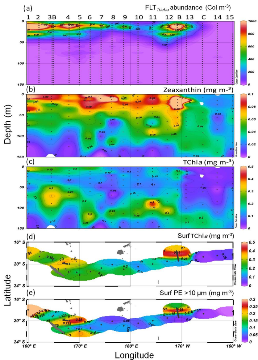
Figure 4. Sections from 0 to 150 m of (a) abundance of FTL_{Tricho} ( N m^{-3} ), (b) zeaxanthin and (c) TChl a concentration ( mg m^{-3} ) measured by HPLC. Surface maps of (d) TChl a and (e) PE > 10 \mu m ( mg m^{-3} ). Short transects TChl a HPLC NASA data from pump samples (sampling at 3.2 m depth) at 165^{\circ} E and 170^{\circ} W are included in the mapping. Source: Ocean Data View (sections Schlitzer, R., Ocean Data View, http://odv.awi.de (last access: 20 August 2018), 2016). Station positions are indicated by black circles.
