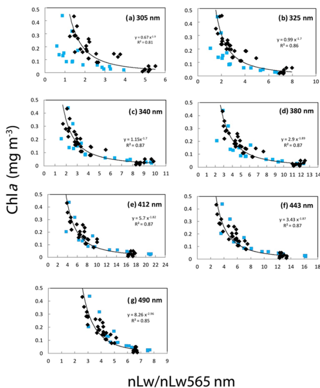
Figure 11. Correlations between the Chl a (fluorimetry) and the ratio of nL_w(\lambda) / nL_w(565\ nm) at different UV and visible wavelengths. Equations and determination coefficient ( r^2 ) of the power law are indicated for each wavelength: (a) 305, (b) 325, (c) 340, (d) 380, (e) 412, (f) 443 and (g) 490 nm. All stations of the OUTPACE (in black) and BIOSOPE (in blue) transect are included.
