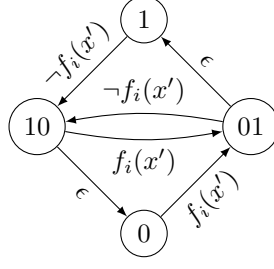
Fig. 1. Automaton of the value change of a component i in the most permissive semantics, following notations of Def. 3. The labels f_i(x') and \neg f_i(x') on edges are the conditions for firing the transitions. \epsilon indicates that the transitions can be done without condition.
