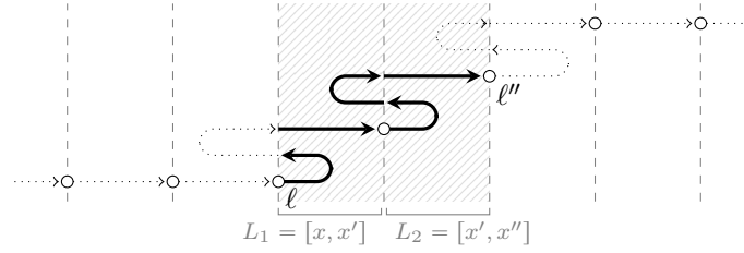
Fig. 10. Two consecutive idempotent loops with the same effect.
