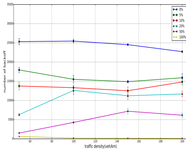
Figure 5: Number of backoffs for different rates of equipped vehicles at different densities, Thr = 1 m, det_r = 40 m
