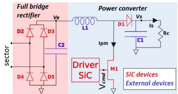
Fig. 1. Electrical schematic of the considered AC/DC demonstrator with a full bridge rectifier and a boost converter.
