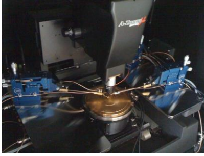
Fig. 2. Semi-automatic probe-station with 3 micromanipulators
