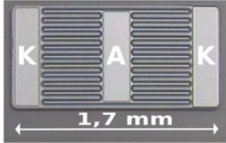
Fig. 8. Top view of the manufactured diode with a width junction of 21.7 mm and a length junction of 10 \mu m.
