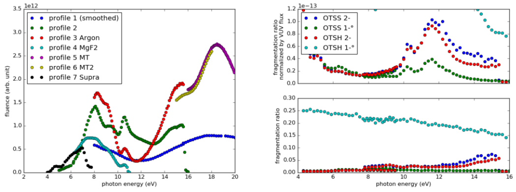
Figure S5 – (Left) Various SOLEIL synchrotron flux profiles depending on the date and the filters used. (Right) Comparison between OT fragmentation ratios with (upper panel) and without normalization by SOLEIL flux (lower panel).
