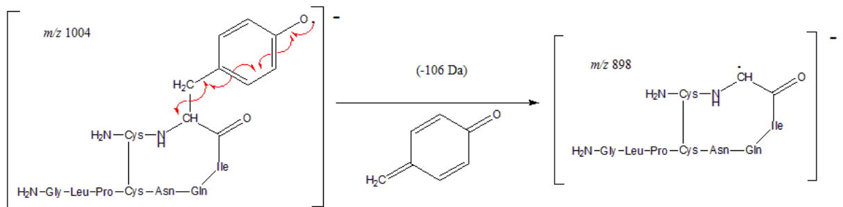
17 Scheme S2 - Proposed mechanism for the loss of Tyrosine side-chain from [OTSS] ^{\bullet-}
