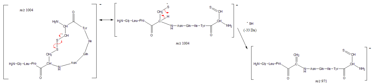
13 Scheme S1 - Proposed mechanism for the loss of \text{SH}^* from [OTSS] ^{\bullet-}
