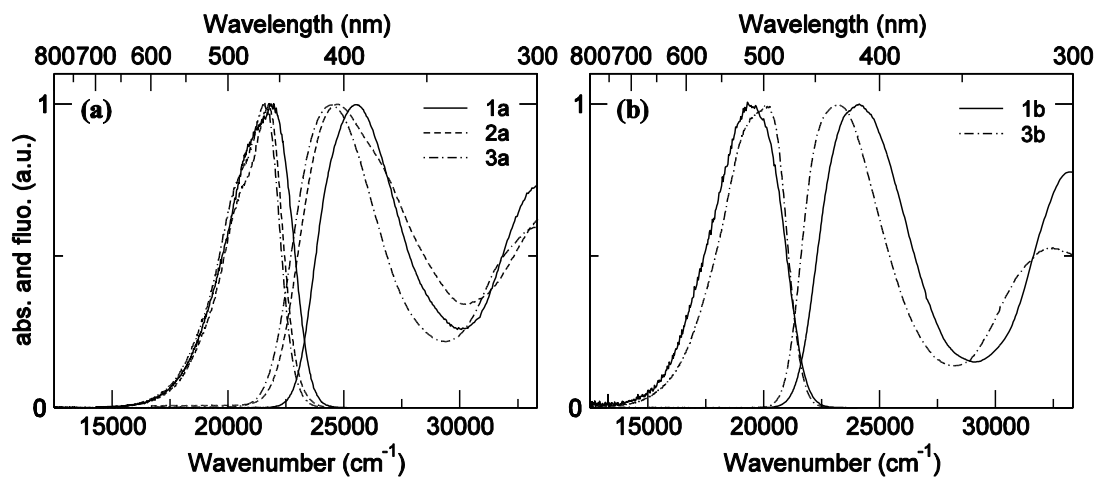
Figure 2: Normalized absorption and fluorescence spectra of (a) 1a-3a in toluene; (b) 1b, 2b in toluene.
