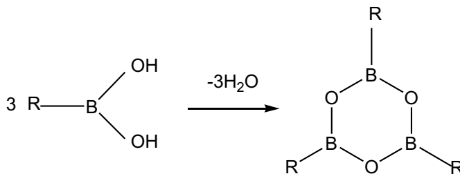
Fig. 2. Synthetic route towards generic compounds Bx .
