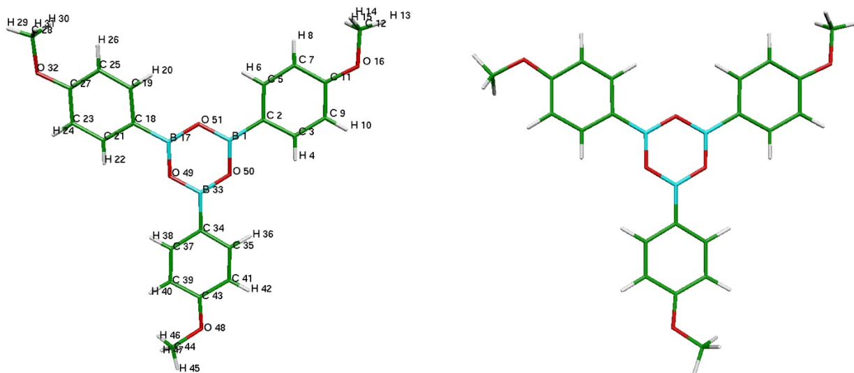
Fig. 5. (left) Molecular geometry of compound B1 as obtained from X-Ray measurements showing atomic numbering. (right) Calculated optimized geometry of boroxine derivative B1 .
