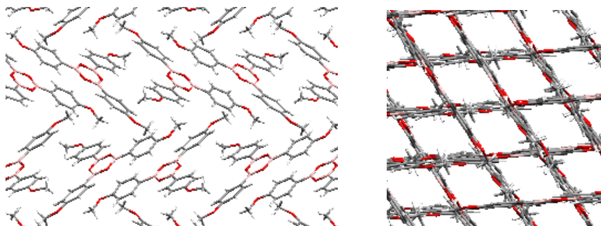
Fig. 4. Packing diagram as obtained from X-Ray measurements on compound B1 : (left) view along the a axis, the b axis is horizontal and the c axis vertical and (right) view of molecular sheets.
