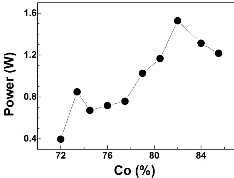
Figure S5. Si-SiO_2//W(3)/Co_xTb_{1-x}(3.5)/AlOx(3) : The electrical power consumption to switch the magnetization at room temperature of a Si-SiO_2//W(3)/Co_xTb_{1-x}(3.5)/AlOx(3) hall bar as a function of Cobalt concentration. The current channel dimensions are length L=100\ \mu\text{m} , and width of w=20\ \mu\text{m} .
