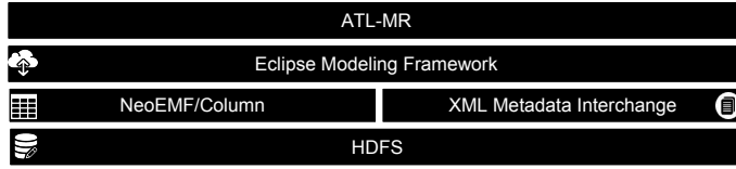
Figure 7: NEOEMF: a general view and architecture
