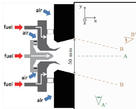
Fig. 1 Top view of the injection device positioned at the entrance of the combustion chamber, showing the two injection stages (pilot: light gray, take-off: dark gray). A laser sheet (A) illuminates the (x,z) plane in the center of the chamber to allow the observation (A') of the fuel droplets Mie scattering signal. An expanded laser beam (B) is sent in the injector hole to visualize (B') the fuel spray near the pilot fuel nozzle. From [9].
