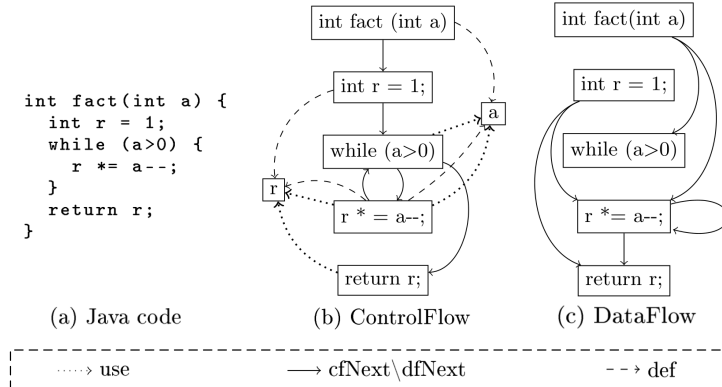
Figure 2: ControlFlow2DataFlow transformation example
