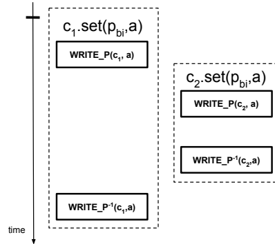
Figure 6: Fail scenario of two concurrent calls on a 1-to-1 bidirectional reference. After both updates finish, they leave the system in an inconsistent state where, c_1 \xrightarrow{p} \emptyset , c_2 \xrightarrow{p} a , and a \xrightarrow{p} c_1
