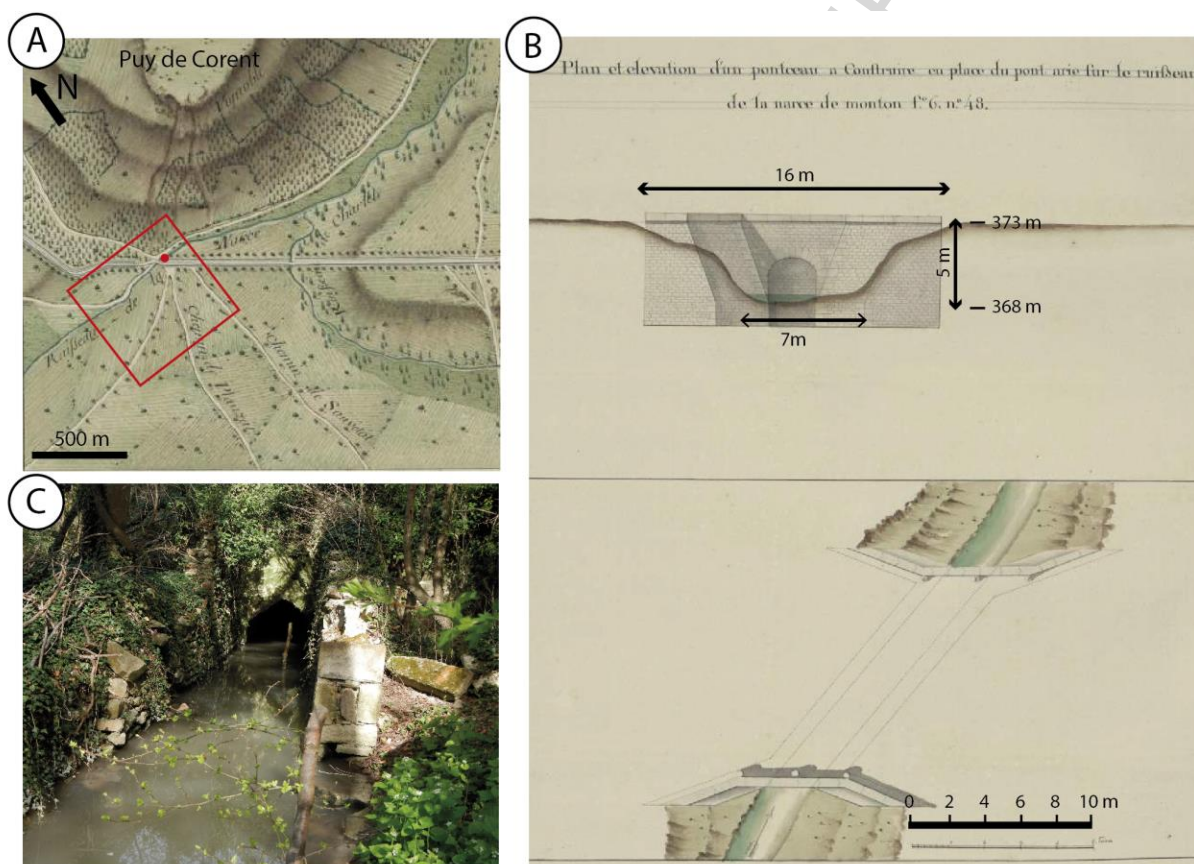
Figure 5. (A and B) Extracts from the XVIII th Century road Atlas de Trudaine, depicting the threshold area (red frame in A), and showing the cross sectional morphology of the still uncovered outlet before the construction of a bridge (B). Altitudes were extracted from current topography, see Fig. 4-E. (C) Current situation of the gallery outlet (red point in A).
