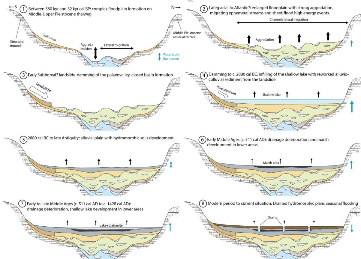
Figure 11. Reconstruction of main hydro-sedimentary phases in the evolution of the basin since the Upper Pleistocene. For sedimentary units colors, see Fig. 6.
