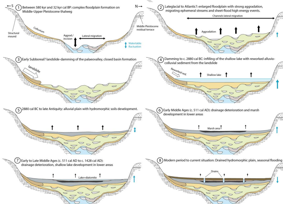
Figure 11. Reconstruction of main hydro-sedimentary phases in the evolution of the basin since the Upper Pleistocene. For sedimentary units colors, see Fig. 6.
