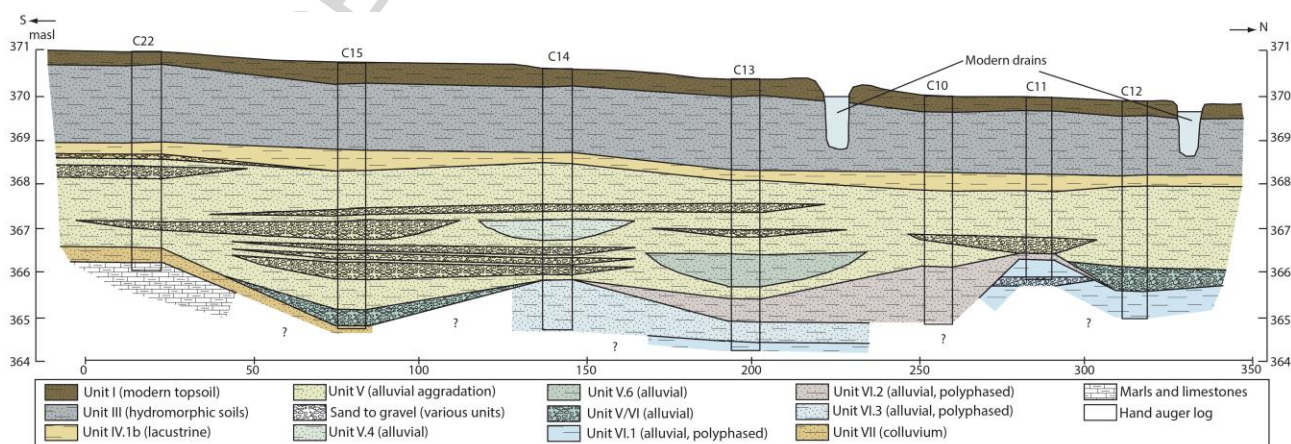
Figure 7. Cross-section 2. For location, see Fig. 3.
