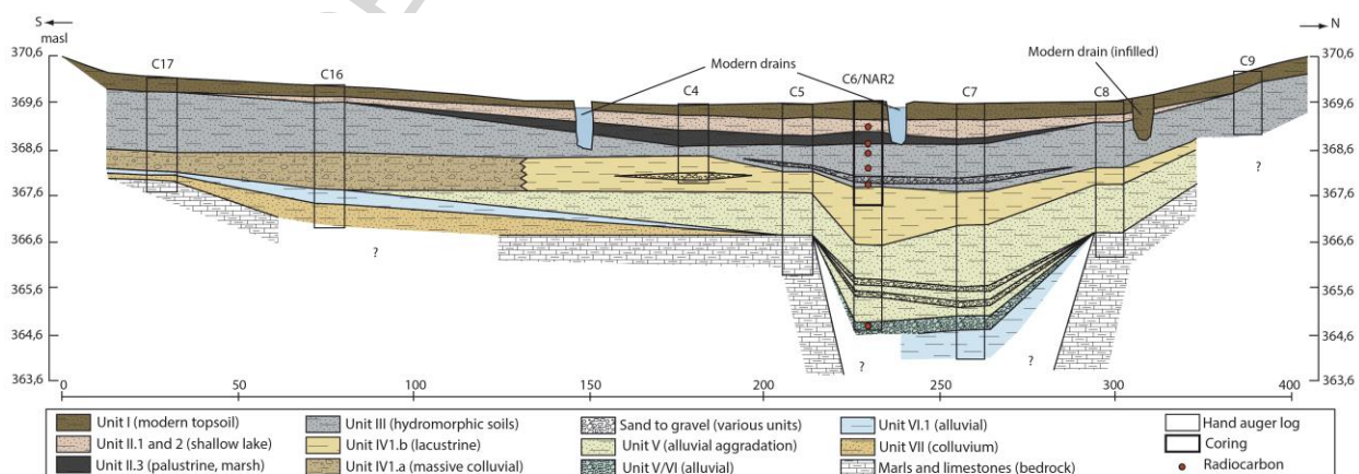
Figure 6. Cross-section 1 (for location, see Fig. 3).
