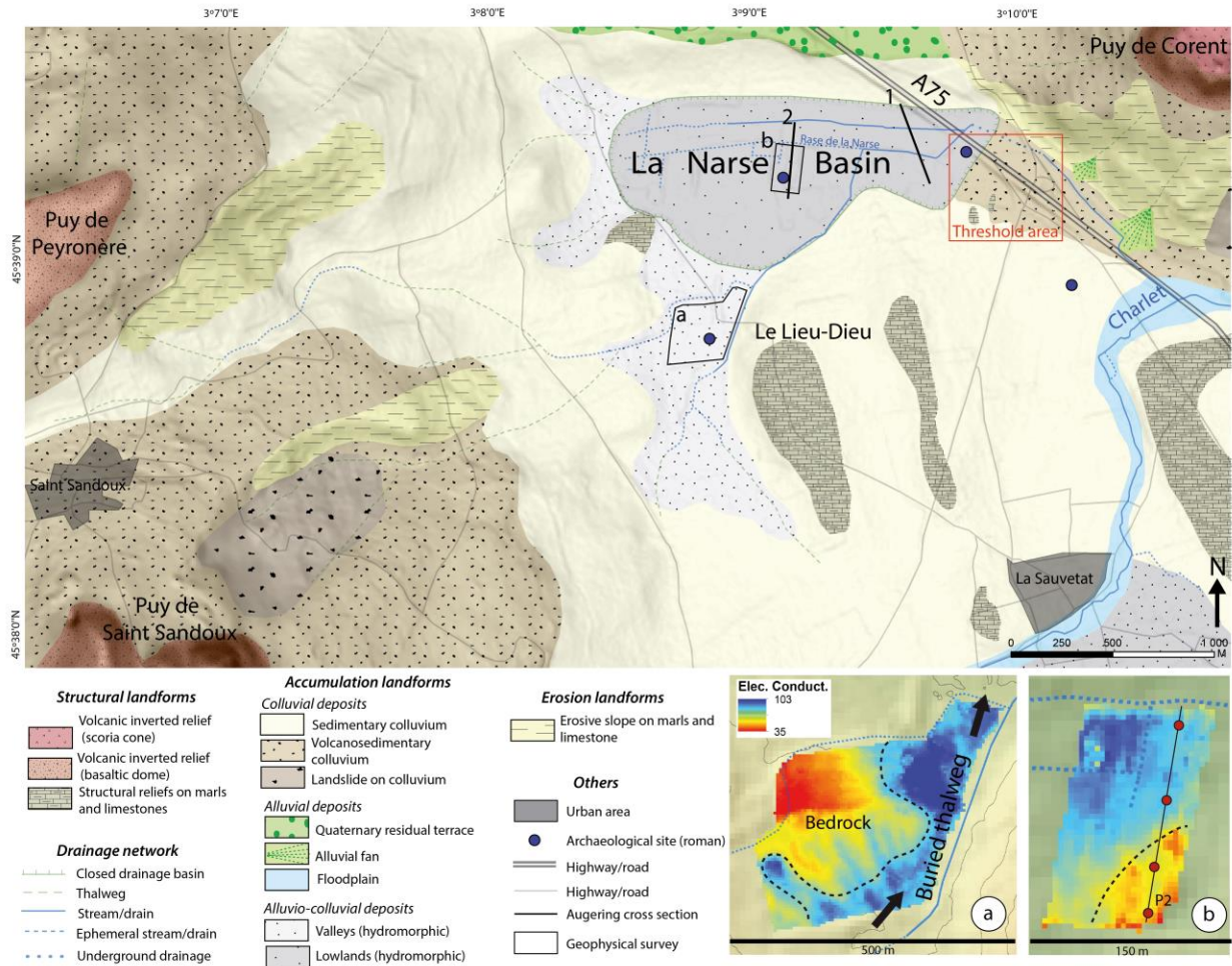
Figure 3. Simplified geomorphological map of the study area. Frames a) and b) correspond to geophysical surveys (electrical conductivity) located on the main map. The red frame represents the geomorphic threshold area.
