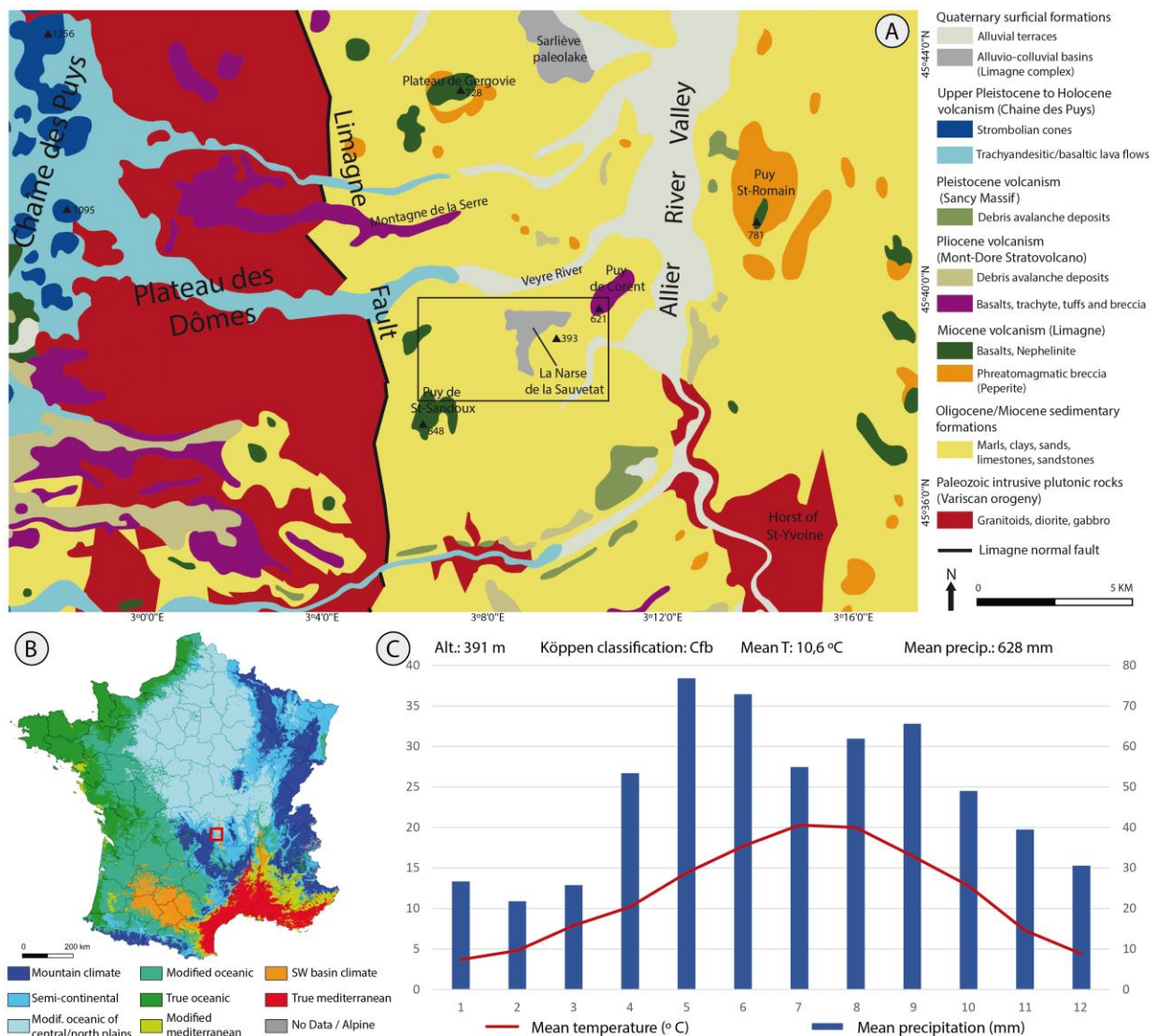
Figure 2. A) Simplified geological map of the study area, modified from BRGM geological map n°717 (Veyre-Monton, in progress). The black frame represents the study area, detailed in Fig.3. B) Location of the study area (red square) in a France “climate type” map (Joly et al., 2010). C) Precipitation and temperature data of the study area (data Météo-France).
