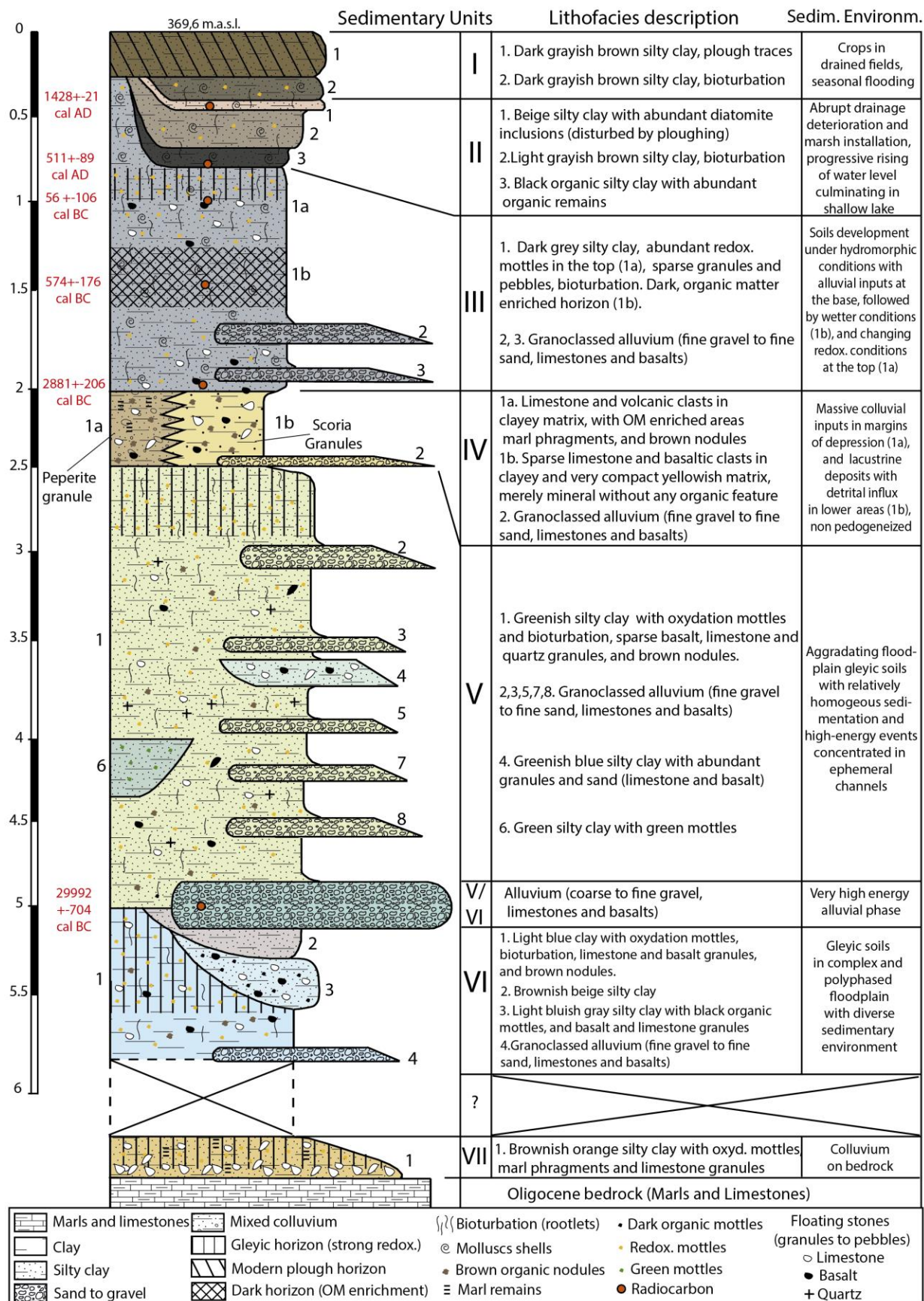
Figure 8. Synthetic stratigraphic column of La Narse de la Sauvetat basin.
