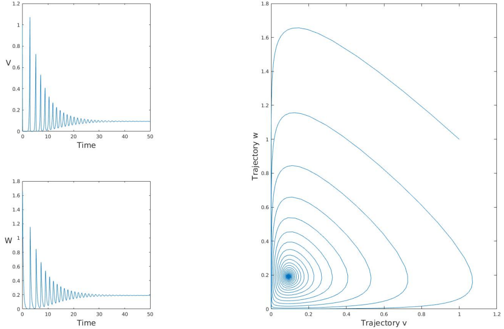
Figure 7: Trajectories of the monomeric concentrations v and w for the two-polymer model for k = 35 , a = b = 1 and \frac{kM}{1+k} < P_0 < kM .
