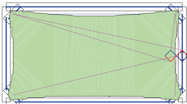
Fig. 7. Workspace of the CDPR grasping the guide
