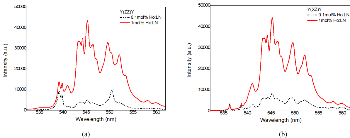
Fig. 3 – Spectra as a function of wavelength of 0.1 and 1% mol Ho doped LN (a) Y(ZZ)Y configuration; (b) Y(XZ)Y configuration
