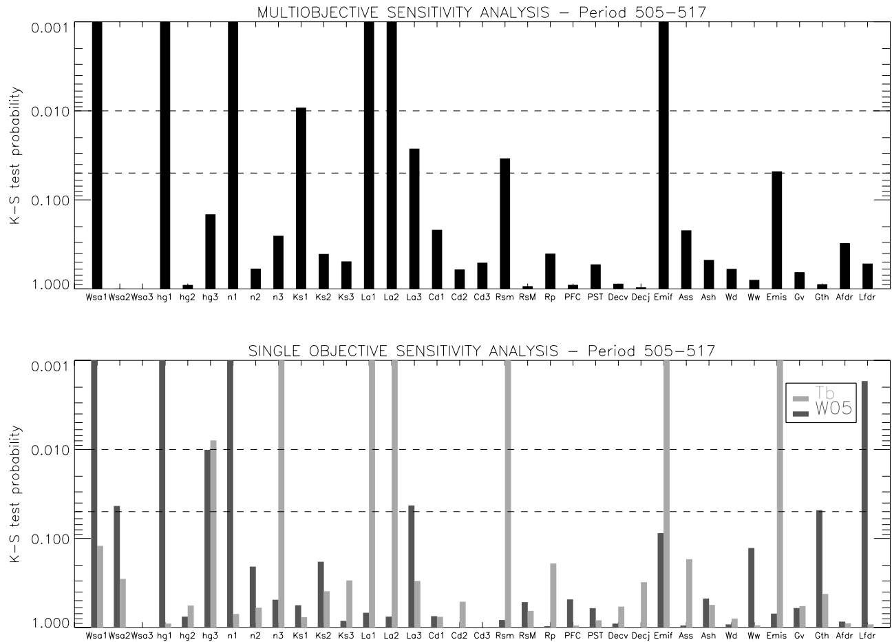
Figure 6. Same as Figure 5, but for period DOE 505–517.
