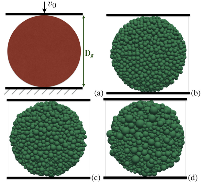
Fig. 2. Schematic representation of diametrical compression test (a), and snapshots of granules composed from 5000 primary spherical particles before diametrical compression for (b) \alpha = 1 ; (c) \alpha = 2 , and (d) \alpha = 5 .
