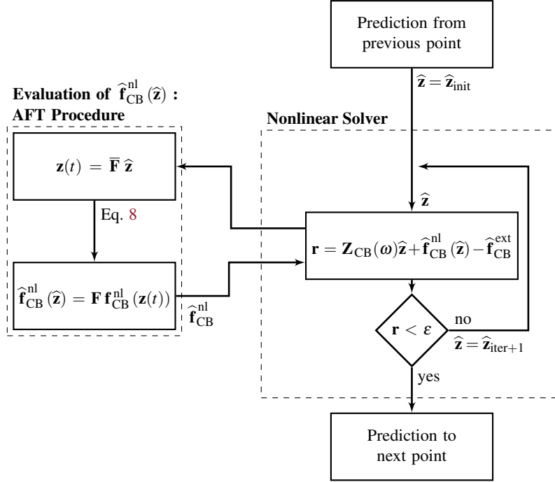
Figure 1. HBM procedure of the reduced system
