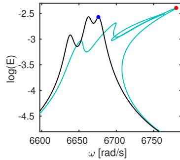
(a) Forced responses associated with the frequency range of interest
