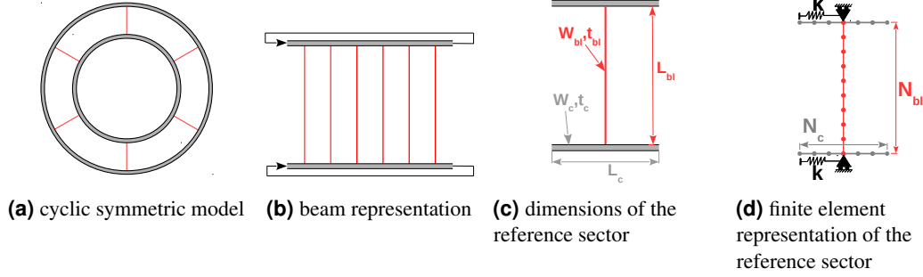
Figure 2. Stator vane model
