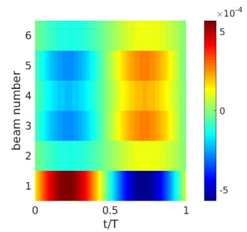
(c) Nonlinear time evolution of the transversal DOF at the middle of each beam: reduced nonlinear system F=0.6N
