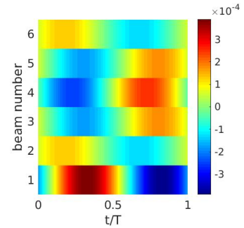
(c) Linear time evolution of the transversal DOF at the middle of each beam (●)
