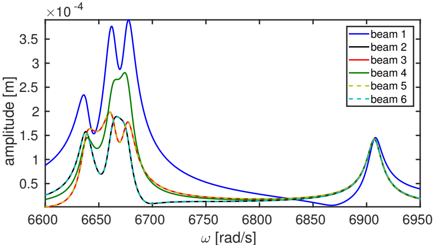
Figure 4. Linear forced response of the system for F=1N
