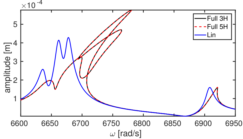
Figure 6. Comparison of the results obtained with 3 and 5 harmonics in the HBM on the beam 1 with F=1.1N
