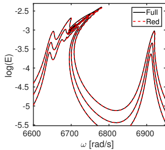
(a) Forced responses of the system
