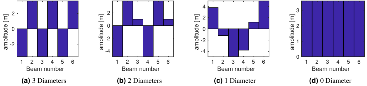
Figure 3. Mode shapes of the first flexural mode family
