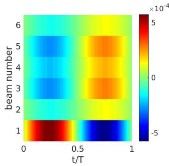
(b) Nonlinear time evolution of the transversal DOF at the middle of each beam: full nonlinear system F=0.6N
