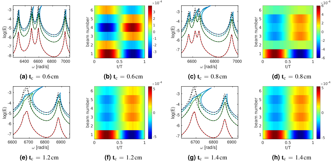
Figure 10. Influence of the thickness of the rings (Linear: - -, Nonlinear: 0.1N , 0.5N , 0.8N , 1.1N )
