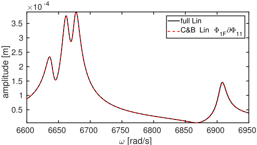
Figure 5. Comparison of the results obtained with reduction on beam 1
