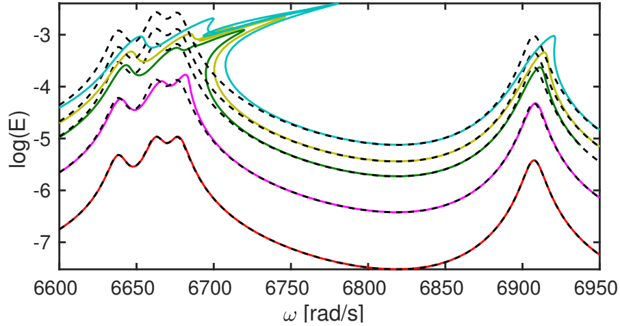
Figure 7. Pulsation-Energy diagram of the full nonlinear system for several forcing amplitudes (Linear: --, Nonlinear: 0.1N , 0.3N , 0.6N , 0.8N , 1.1N )
