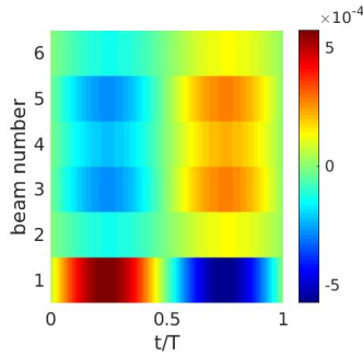
(b) Nonlinear time evolution of the transversal DOF at the middle of each beam (●)
