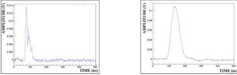
Fig. 2. The examples of output pulses generated by PMT (left) and pulse-shaping amplifier (right) in XEMIS1
