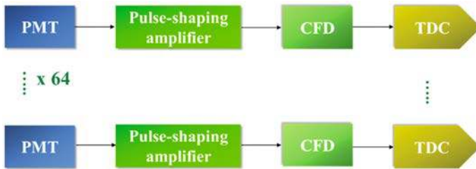
Fig. 3. Preliminary design of XEMIS2 scintillation signal detection chain
