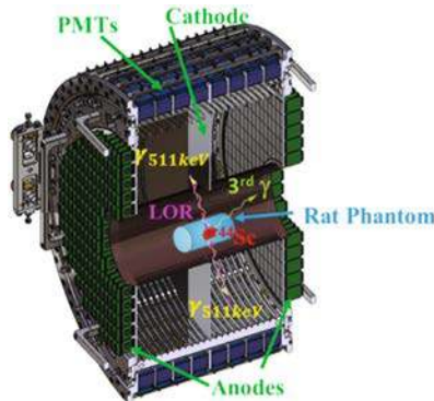
Fig. 1. The active zone of the XEMIS2 prototype
