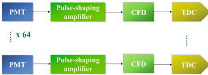
Fig. 3. Preliminary design of XEMIS2 scintillation signal detection chain
