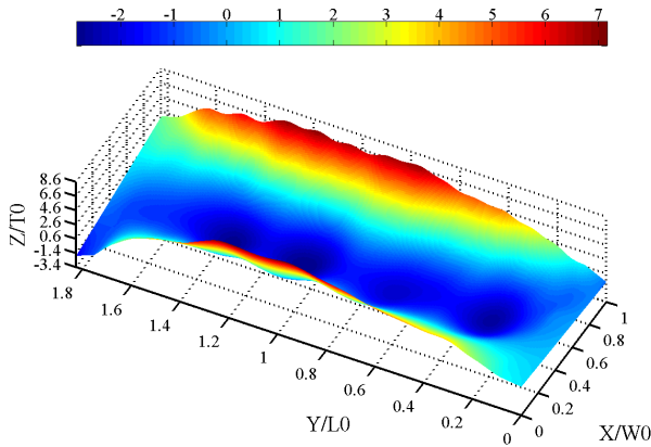
Fig. 6: Initial imperfections for \bar{\sigma} = 1.5\text{MPa}
