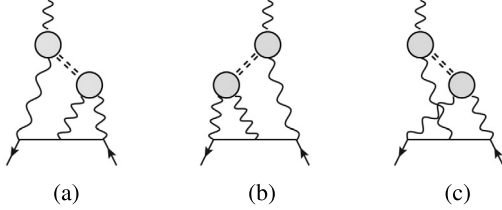
Fig. 2. Scalar meson exchange (dotted lines) to Light-by-light scattering contribution to a_\mu . The wavy lines represent photon. The shaded blob represents form factors. The first and second diagrams contribute to the function T_1 , and the third to the function T_2 defined in Eq. (3.11).
