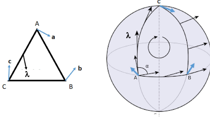
FIG. 3: Two closely related, though intrinsically different, random games: the game on the left hand side is constrained by the Bell's inequality, while the one on the right hand side is not necessarily constrained by the inequality. In both games we have reference unit vectors, labelled respectively as \vec{a} , \vec{b} and \vec{c} , drawn at each one of the vertices, labelled as A , B and C , of a triangle. In the game on the left the triangle is drawn on a plane surface and the reference unit vectors are contained within the plane, while in the game on the right the 'triangle' is defined on the surface of a sphere by segments of three great circles and the three reference unit vectors lay within the corresponding tangent planes. Two copies of a randomly oriented unit vector \vec{\lambda} are generated at random at the center of one of the three segments of the triangle with density of probability \rho(\vec{\lambda}) , and detected, respectively, at the two detectors located at the ends of the segment. In the game on the left the vector \vec{\lambda} is contained within the plane surface, while in the game on the right the vector \vec{\lambda} is tangent to the sphere. The binary responses of the detectors are locally defined by parallelly transporting the unit vector \vec{\lambda} along the segment of the triangle to its end, and comparing its orientation to the orientation of the corresponding reference unit vector: A(\vec{a}, \vec{\lambda}) = \text{sign}(\vec{a} \cdot \vec{\lambda}) , B(\vec{b}, \vec{\lambda}) = \text{sign}(\vec{b} \cdot \vec{\lambda}) , C(\vec{c}, \vec{\lambda}) = \text{sign}(\vec{c} \cdot \vec{\lambda}) . It is then straightforward to prove the Bell's inequality for the game on the left, since for any settings \vec{a}, \vec{b}, \vec{c} and any random vector \vec{\lambda} the following equality holds: \left| A(\vec{a}, \vec{\lambda}) \cdot B(\vec{b}, \vec{\lambda}) + A(\vec{a}, \vec{\lambda}) \cdot C(\vec{c}, \vec{\lambda}) \right| = 1 + B(\vec{b}, \vec{\lambda}) \cdot C(\vec{c}, \vec{\lambda}) . Therefore, after integrating over the whole space of possible hidden configurations: \left| \int d\vec{\lambda} \rho(\vec{\lambda}) \left[ A(\vec{a}, \vec{\lambda}) \cdot B(\vec{b}, \vec{\lambda}) + A(\vec{a}, \vec{\lambda}) \cdot C(\vec{c}, \vec{\lambda}) \right] \right| \leq \int d\vec{\lambda} \rho(\vec{\lambda}) \left| A(\vec{a}, \vec{\lambda}) \cdot B(\vec{b}, \vec{\lambda}) + A(\vec{a}, \vec{\lambda}) \cdot C(\vec{c}, \vec{\lambda}) \right| = \int d\vec{\lambda} \rho(\vec{\lambda}) \left| A(\vec{a}, \vec{\lambda}) \cdot B(\vec{b}, \vec{\lambda}) + A(\vec{a}, \vec{\lambda}) \cdot B(\vec{b}, \vec{\lambda}) \cdot B(\vec{b}, \vec{\lambda}) \cdot C(\vec{c}, \vec{\lambda}) \right| = 1 + \int d\vec{\lambda} \rho(\vec{\lambda}) B(\vec{b}, \vec{\lambda}) \cdot C(\vec{c}, \vec{\lambda}) , and therefore, \left| E^{A,B}(\vec{a}, \vec{b}) + E^{A,C}(\vec{a}, \vec{c}) \right| \leq 1 + E^{B,C}(\vec{b}, \vec{c}) . This proof, nonetheless, does not hold for the random game on the right hand side, since the orientation of a vector \vec{\lambda} parallelly transported along the closed contour of the triangle ABC gets rotated by a geometric phase \alpha due to the curvature of the sphere. In fact, in the game on the right the three bipartite correlations are constrained by the inequality \left| E^{A,B}(\vec{a}, \vec{b}) + E^{A,C}(\vec{a}, \vec{c}) \right| \leq 1 + E^{B,C}(\vec{b}, \hat{\mathcal{R}}_\alpha \vec{c}) , where \hat{\mathcal{R}}_\alpha \vec{c} denotes the rotation of vector \vec{c} by an angle \alpha .
