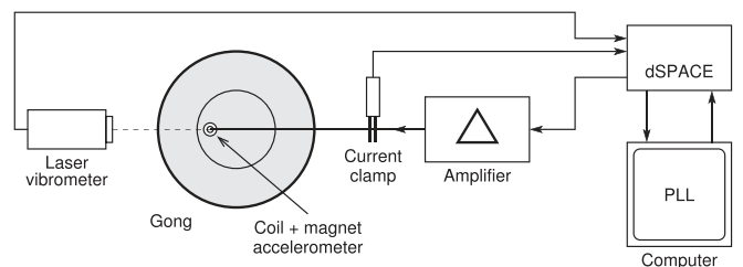
FIG. 2. Setup for experiment A (PLL measurements, single nonlinear mode excited).
