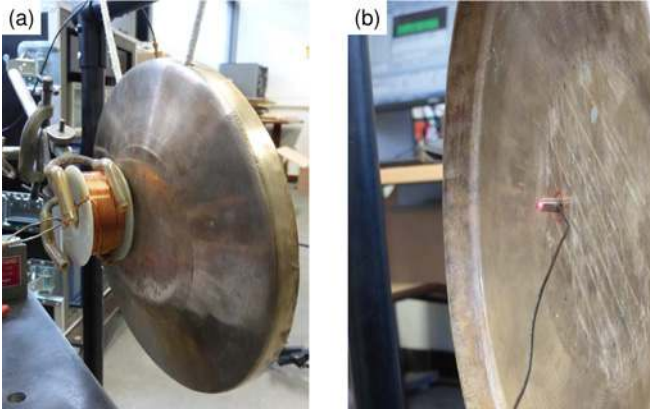
FIG. 3. (Color online) Instrumentation of the gong. (a) Front of the xiaolu gong with magnet-coil system. (b) Back of the gong with the accelerometer co-localized with the laser vibrometer.
