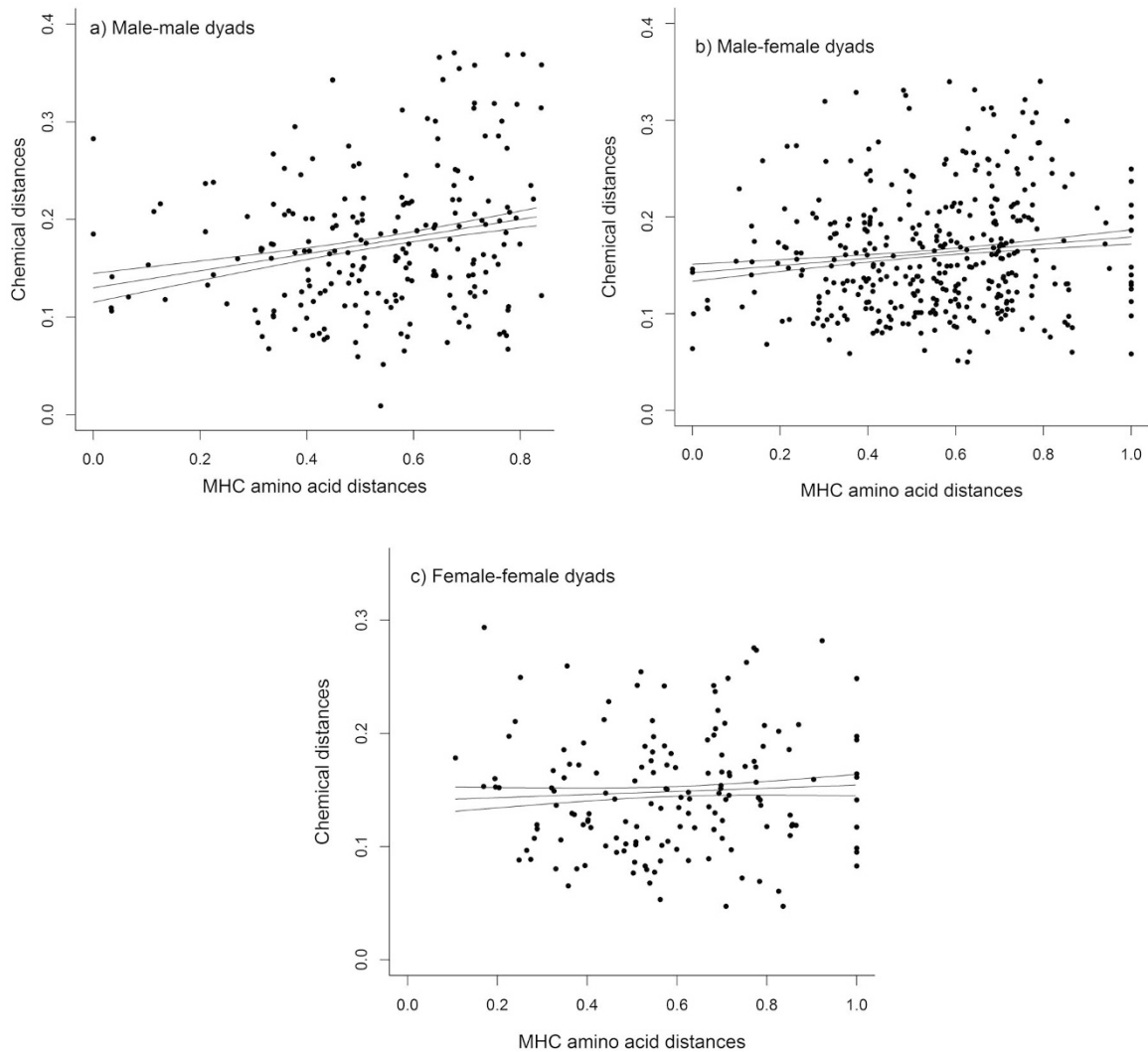
Figure 2 | Relationship between MHC amino-acid distances and chemical distances (as described by Euclidean distances) in (a) male-male dyads, (b) cross-sex dyads, and (c) female-female dyads. Solid lines are linear model predicted values and SE.
