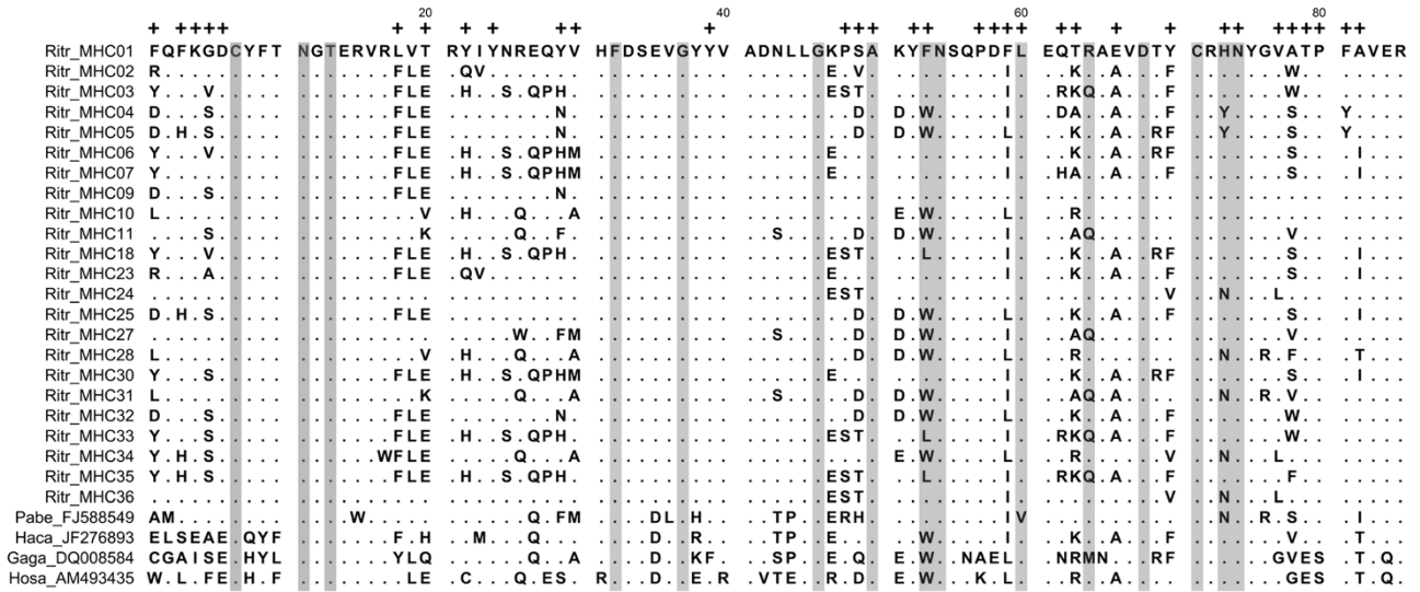
Figure 1 | Amino acid alignment of MHC Class II DRB alleles isolated from black-legged kittiwakes. Dots indicate matching amino acids relative to Ritr_MHC01 and shaded areas indicate conserved residues as outlined in 50 . Plus signs above alignment correspond to putative antigen binding sites as inferred from 46 . Additional species and their associated GenBank accession numbers included in the alignment are Pachyptila belcheri (FJ588549), Halobaena caerulea (JF276893), Gallus gallus (DQ008584) and Homo sapiens (AM493435).
