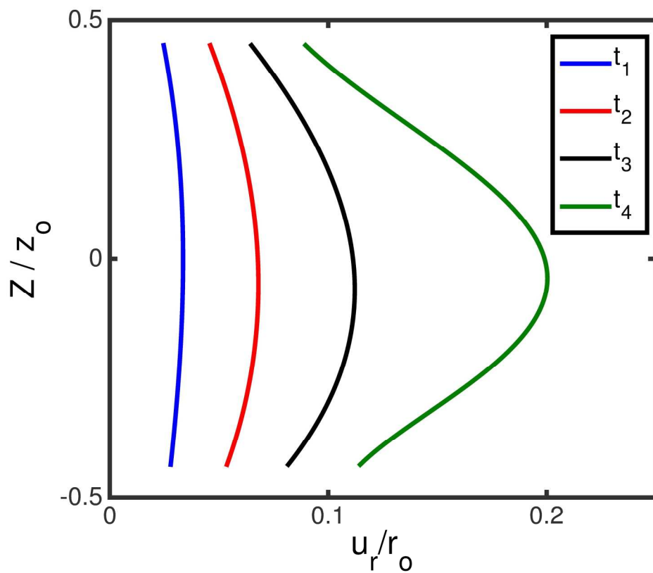
FIG. 10: Procedure Test B. Normalized out-of-plane displacement u_r/r_0 of each marker versus the normalized axial coordinate Z/Z_0
