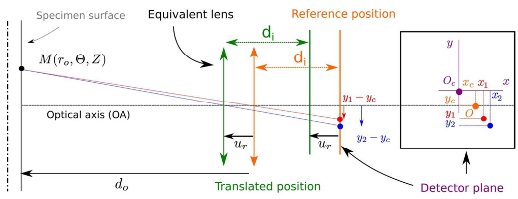
FIG. 7: Procedure Test B. Scheme of the experiment used to calibrate the optical system parameters: d_o, x_c, y_c .
