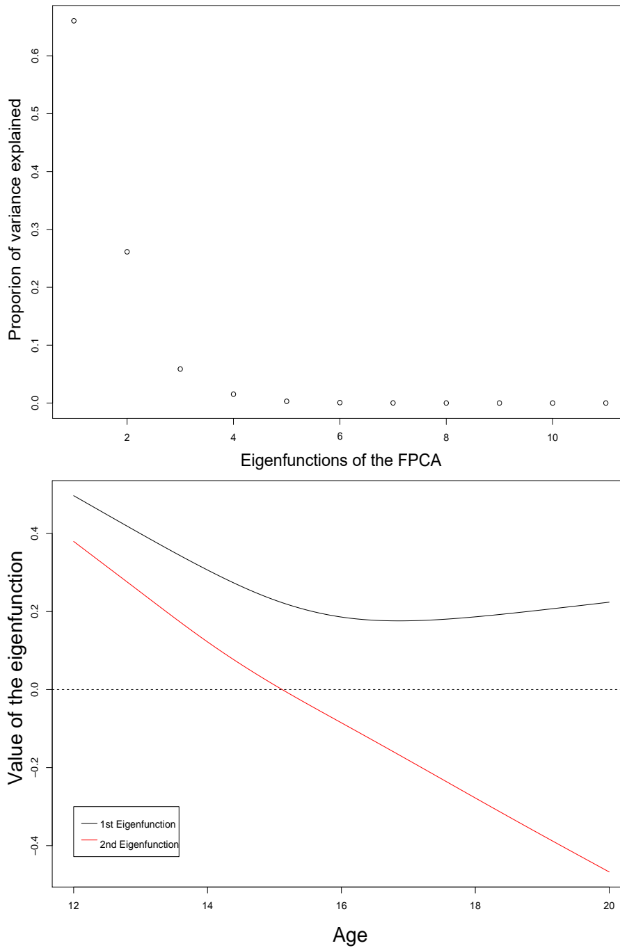
Figure A1. Results of the functional principal component analysis (FPCA) on the progression curves. (Top) proportion of variance explained by each eigenfunction. With only two eigenfunctions, one can express about 90% of the total variance of the data set; (Bottom) values of the two first eigenfunctions. Eigenfunctions are orthogonal to each other and display the main modes of variation of the curves. The first eigenfunction mainly informs about differences at young ages, while the second focuses on the opposition between speeds at young and older ages.
