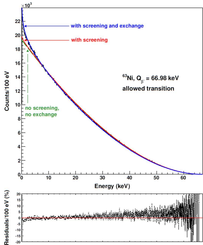
Fig.3. Beta spectrum of an electroplated ^{63}\text{Ni} source measured with a metallic magnetic calorimeter (“rugged” black line), compared with theoretical spectra without any correction for atomic effects, with screening correction and with screening and exchange effects. The lower part of the figure shows the residuals between experiment and the full theory including screening and exchange effects.
