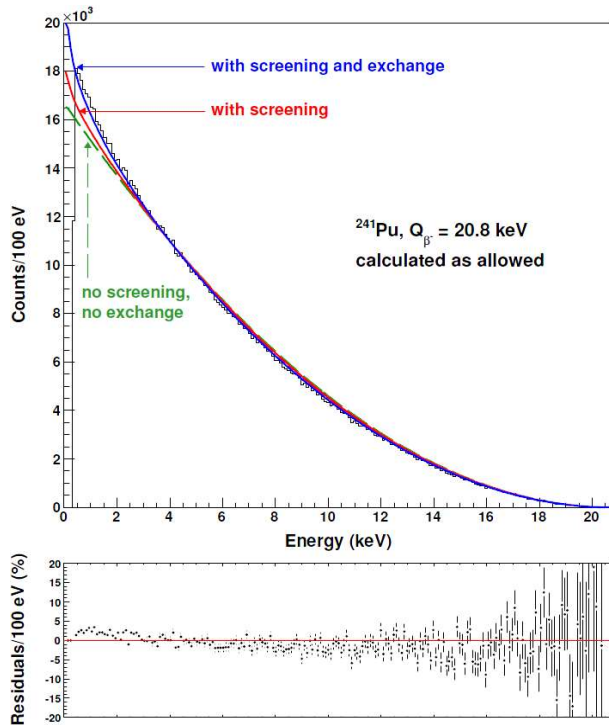
Fig 4. Spectrum of ^{241}\text{Pu} measured with a metallic magnetic calorimeter (thin solid line, histogram), compared with theoretical spectra calculated without any correction for atomic effects, with screening correction and with corrections for screening and exchange effect. The lower part of the figure shows the residuals between experiment and theory with screening and exchange effects.
