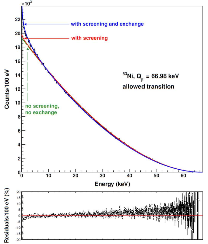
Fig.3. Beta spectrum of an electroplated ^{63}\text{Ni} source measured with a metallic magnetic calorimeter (“rugged” black line), compared with theoretical spectra without any correction for atomic effects, with screening correction and with screening and exchange effects. The lower part of the figure shows the residuals between experiment and the full theory including screening and exchange effects.
