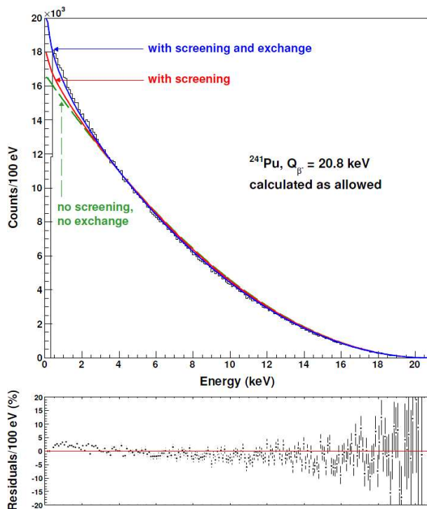
Fig 4. Spectrum of ^{241}\text{Pu} measured with a metallic magnetic calorimeter (thin solid line, histogram), compared with theoretical spectra calculated without any correction for atomic effects, with screening correction and with corrections for screening and exchange effect. The lower part of the figure shows the residuals between experiment and theory with screening and exchange effects.
