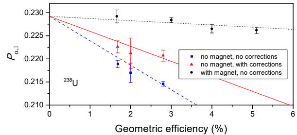
Fig. 2. Emission probability values of the second largest peak in the alpha decay of ^{238}\text{U} , derived from the deconvolution of the spectra taken with magnet (circles) and without magnet, before (squares) and after (triangles) mathematical correction for coincidence effects.
