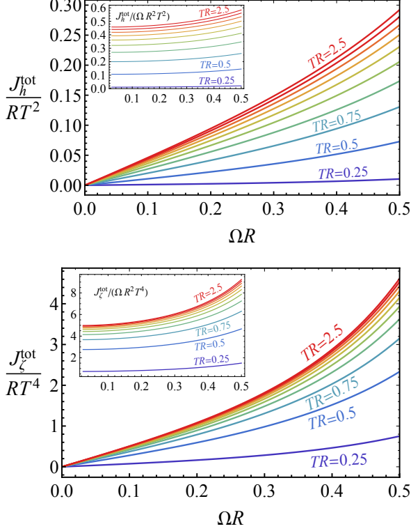
FIG. 2: The total helicity ( s = 1 ) and zilch ( s = 0 ) currents (99) as function of the dimensionless tangential velocity at the boundary R\Omega . The plots show that behavior of the dimensionless quantities J_h^{z,\text{tot}}/(RT^2) and J_\zeta^{z,\text{tot}}/(RT^4) for the same temperature range as in Fig. 1. The insets show the currents divided by the frequency \Omega .
