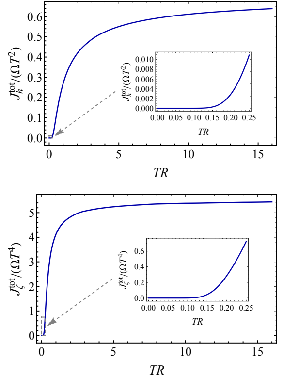
FIG. 3: The dimensionless strength of the helicity ( s = 1 ) and zilch ( s = 0 ) currents (100) in the limit of small angular frequencies \Omega \rightarrow 0 as function of temperature T . The insets show the exponential onset of both currents at small temperatures.
