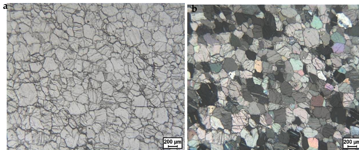
Figure 10. Polarized light images, parallel (a) and crossed (b) polars of A63MA sample.
