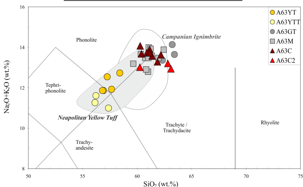
Figure 12. TAS diagram (Le Bas et al. , 1986) glasses (juvenile materials). Neapolitan Yellow Tuff and Campanian Ignimbrite fields are from Rosi and Sbrana (1987), Scarpato et al. (1993), Orsi et al. (1996), Signorelli et al. (1999), Melluso et al. (1995), Civetta et al. (1997), Pappalardo et al. (2002) and Fedele et al. (2008).
