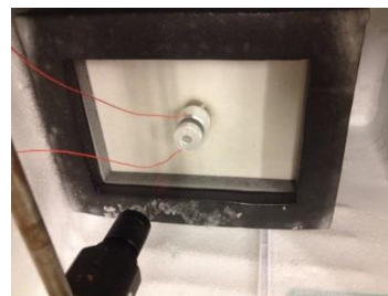
Figure 14 – Study case: bolt-clamped Langevin transducer connected to the plate
